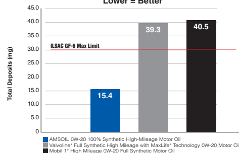
TEOST 33C (ASTM D6335) Lower = Better
