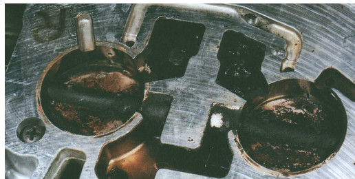
Picture J - Carburetor plates before P.i. treatment
