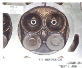
Picture F - Combustion chamber before P.i. treatment
